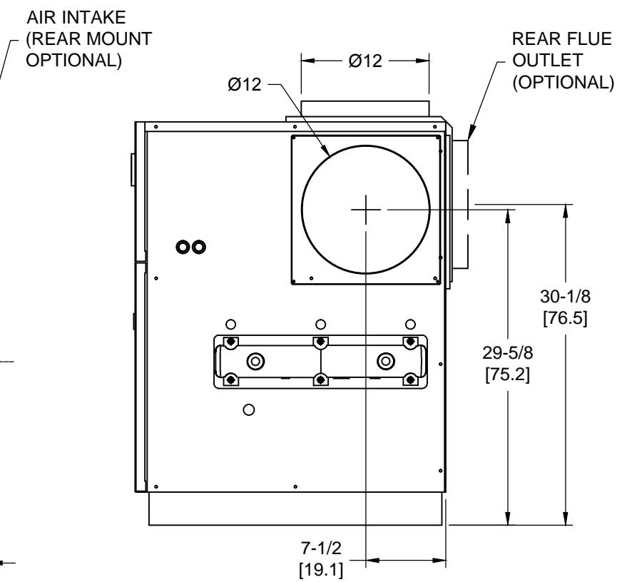
RIGHT VIEW
