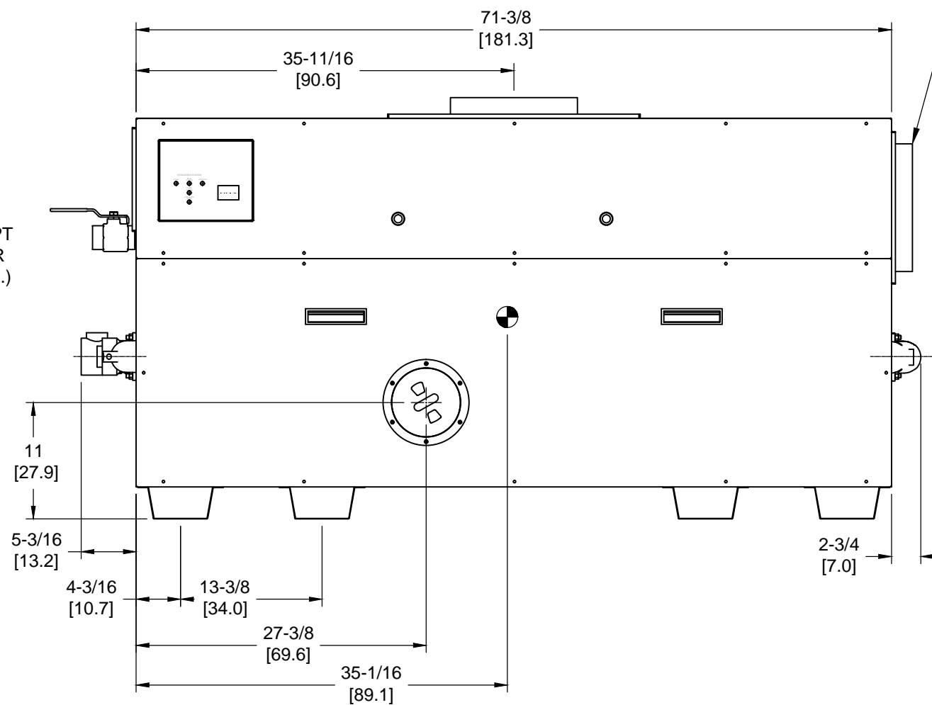
FRONT VIEW
